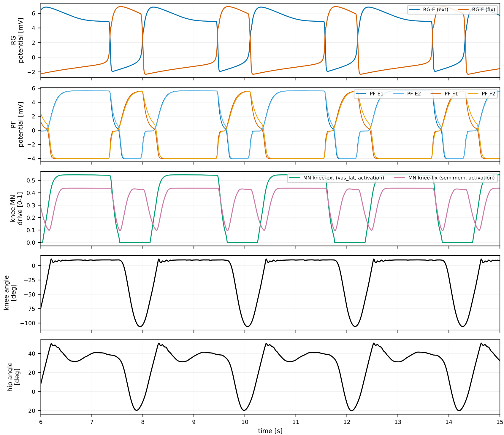
gait2392 spinal SNS - right leg (nap_air, RoM limits + Renshaw 0.5)
